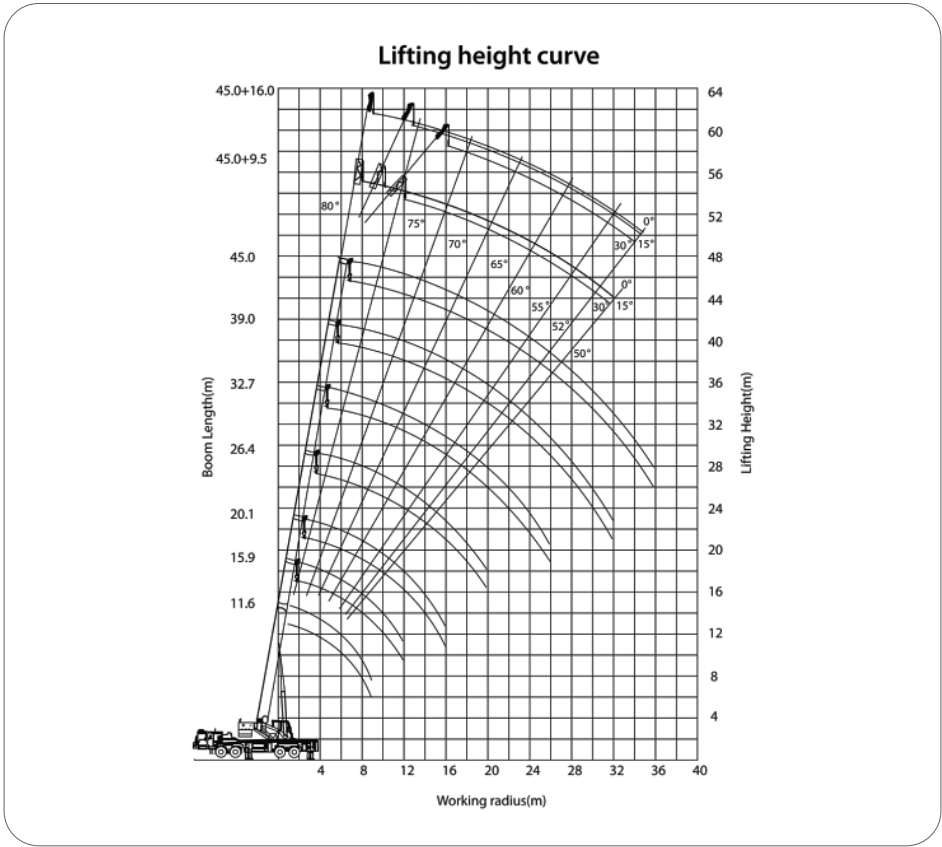
Figure 15: Example of a load chart showing boom height and angle (Photo courtesy of Antar Cranes Services Pte Ltd)
