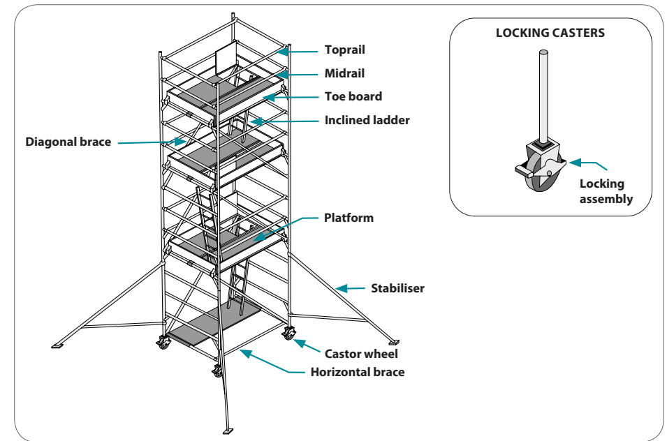
Figure 5: Example of a mobile tower scaffold.
