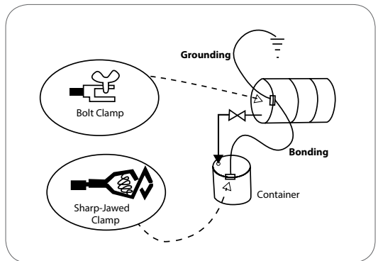
Figure 9: Example of bonding and grounding
