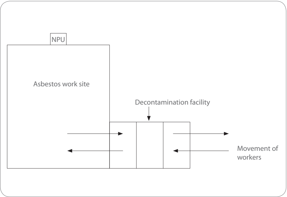
Figure 12: Illustration of a decontamination facility.
