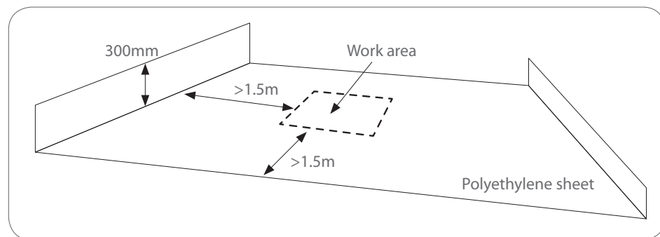
Figure 7: Flooring to be covered with polyethylene sheets at the asbestos work area.
