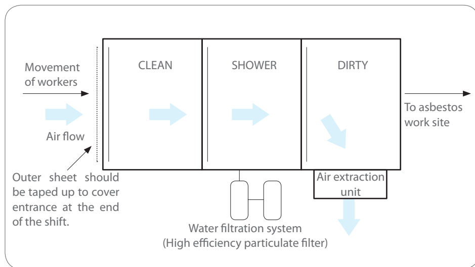
Figure 14: Illustration of a decontamination facility equipped with a high efficiency particulate filter and air extraction unit.
