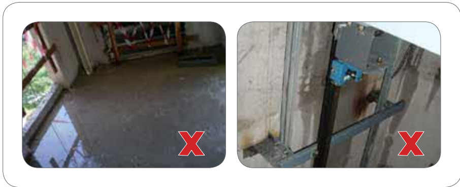
Figure 19: Worker can get electrocuted when he comes into contact with a flooded or damp hoist way.
